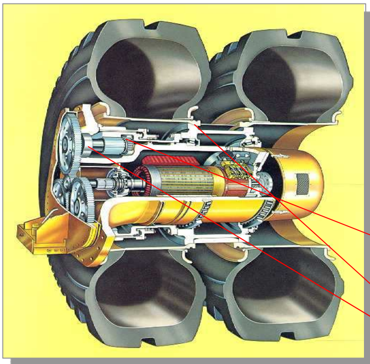
Electric Wheel
