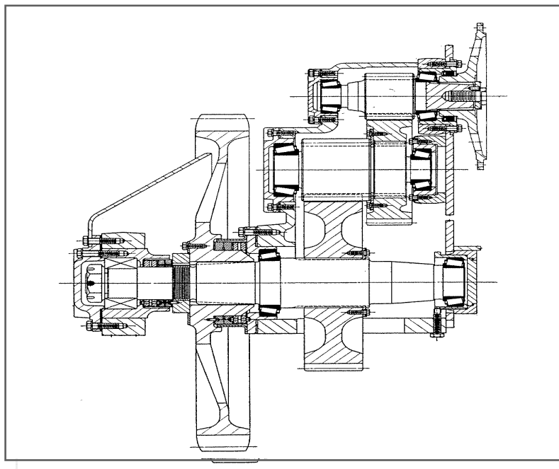
Low-Horsepower Design
